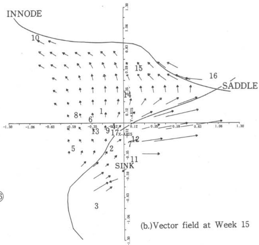
Figure 11. Recovered vector fields at Weeks 0 and 15 via DYNASCAL.
